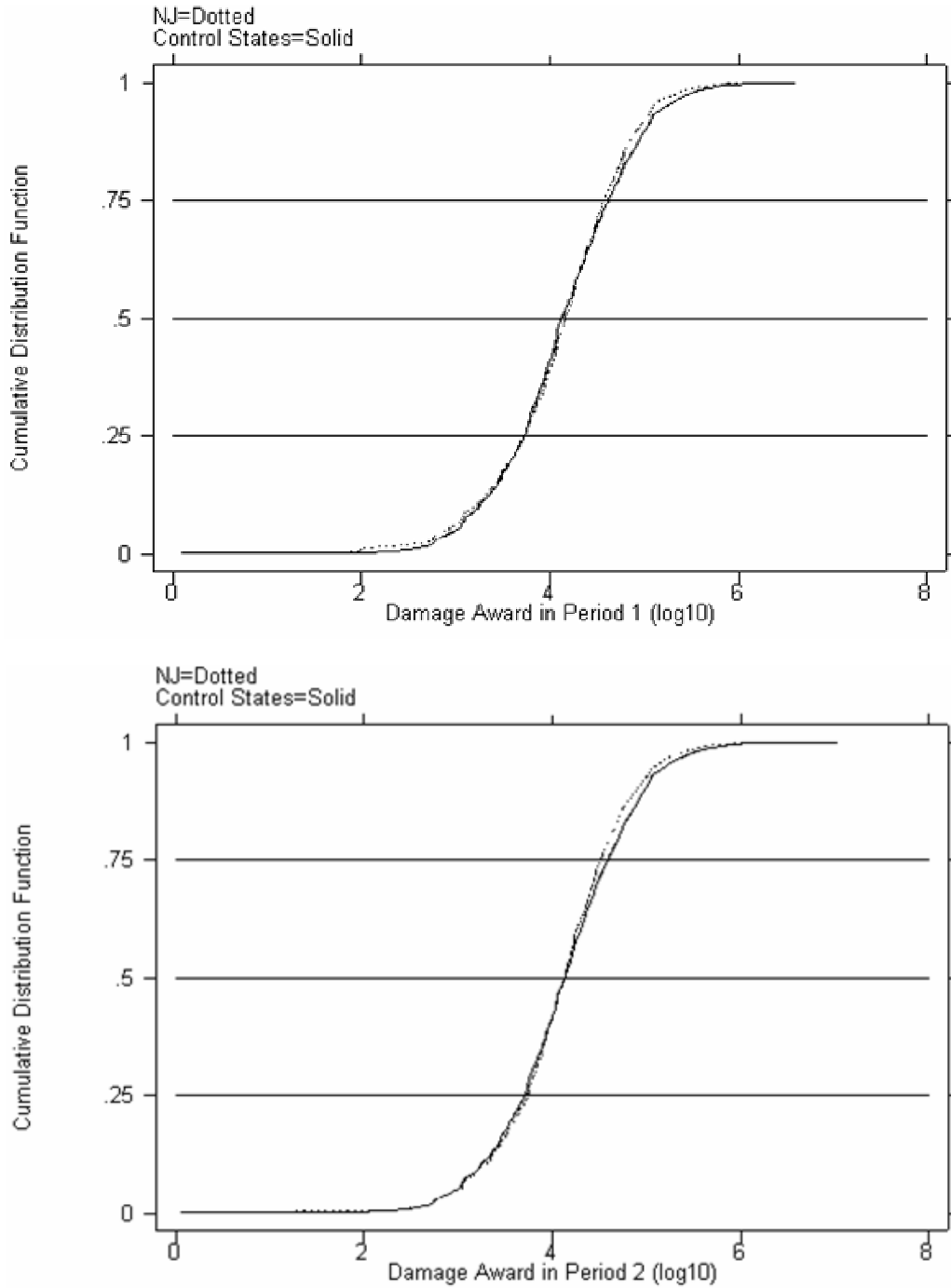
Figure 5 Cumulative Distribution Function Comparison of Damage Awards Period 1 vs. Period 2
