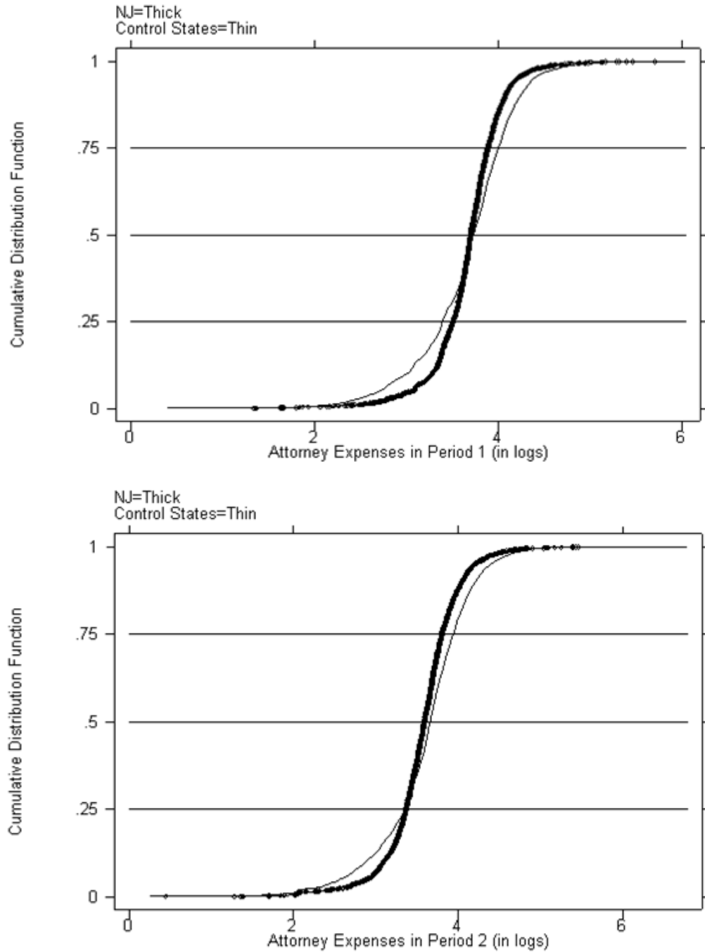
Figure 7 Cumulative Distribution Function Comparison of Attorneys Fees Period 1 vs. Period 2
