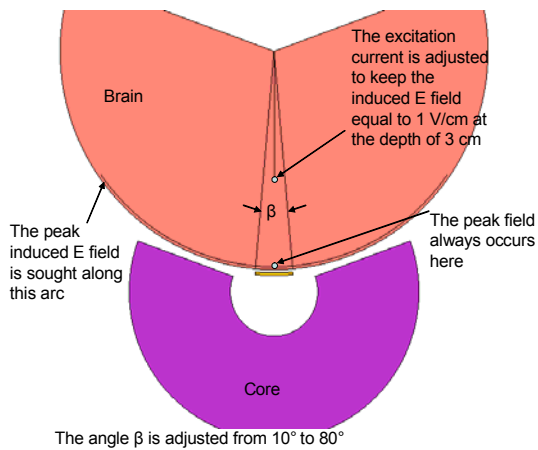
Fig. 5 Changing the angle of the shield conductor reduces the maximum induced field on the scalp.
