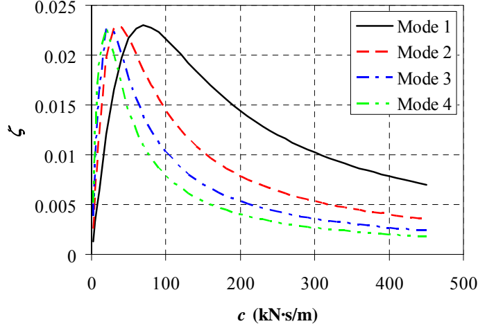
Figure 6.10 Damping supplemented to stay AS16 by dampers of different coefficient
