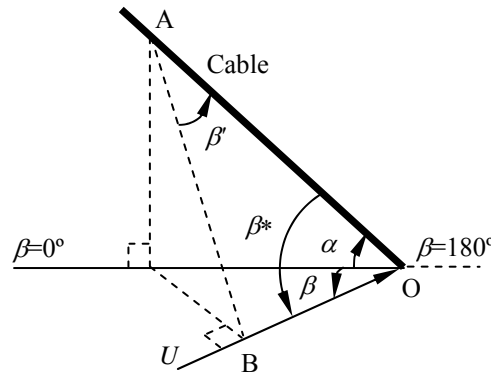
Figure 5.7 Relative wind attack angle
