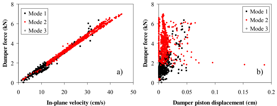
Figure 6.12 Damper force vs. a) anti-nodal cable velocity amplitude and b) damper piston velocity amplitude for stay AS16
