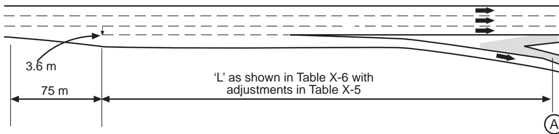
- C - PARALLEL DESIGN
