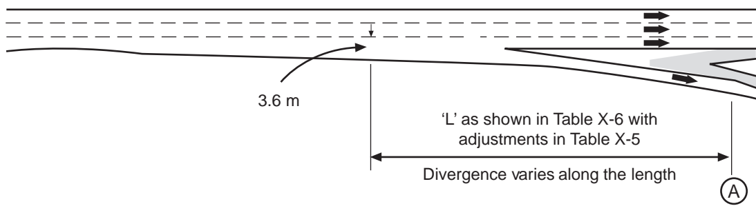
- B - TAPERED DESIGN - CURVILINEAR
